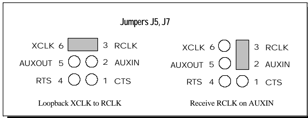
Figure 20 --- RCLK selection
